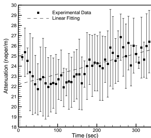
Figure 3. Ultrasonic attenuation in CMT milk, at \text{SCC}=72.5(10^3/\text{ml}) , T = 30^\circ\text{C} and f = 1\text{ MHz} .
