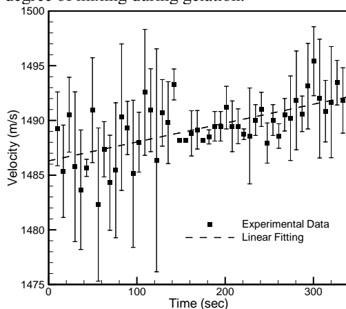
Figure 2. Ultrasonic velocity in CMT milk, at \text{SCC}=72.5(10^3/\text{ml}) , T = 30^\circ\text{C} and f = 1\text{ MHz} .
